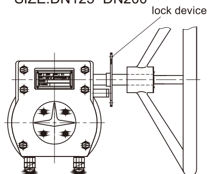
Gear Operation (Standard Type) SIZE:DN125~DN200
